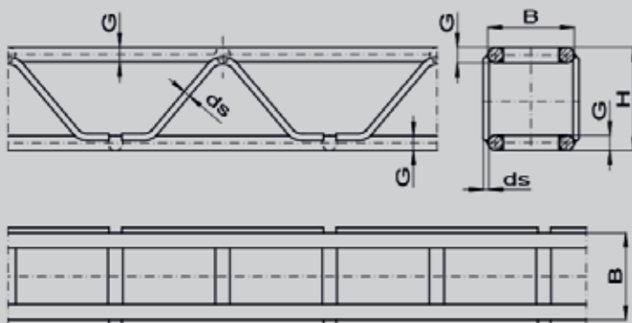
4-Gurt-System/4-bar girder system
