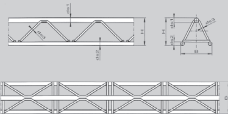
3-Gurt-System/3-bar girder system
